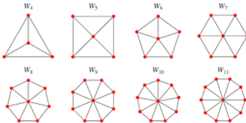
W_n , Wheels with n vertices
