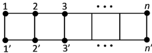
L_n , Ladder with 2n vertices
